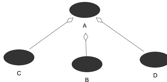
Figure 9: Aggregation is shown with a line adorned by a diamond. The use case most close to the diamond is the containing use case.
