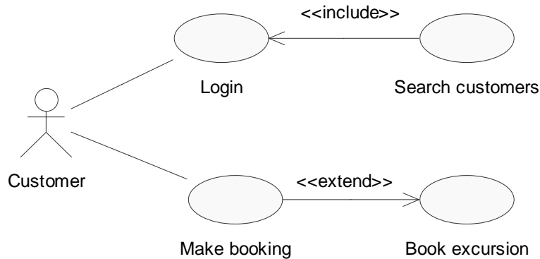
Figure 3: A simple use case model with an <<extend>> and an <<include>> stereotype.
