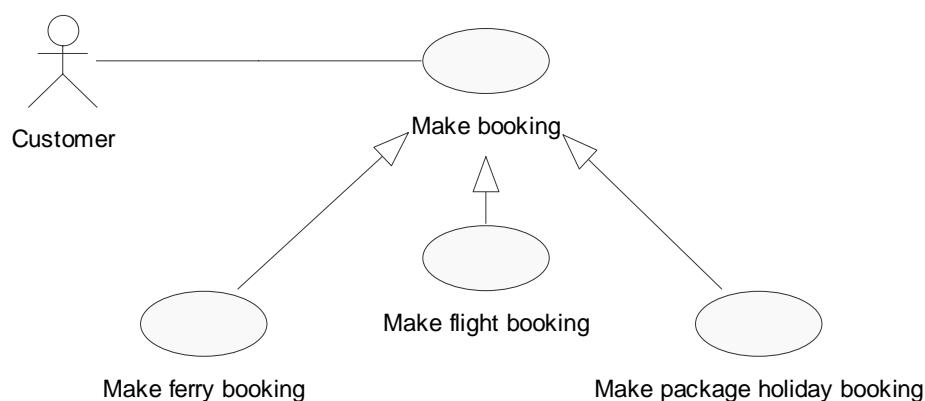
Figure 4: A use case structure where the specialisation association has been employed to add more information about the use case relationships.
