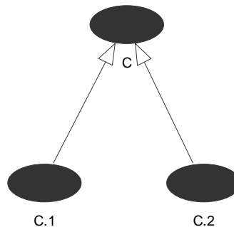
Figure 10: Specialisation (or inheritance, or generalisation) is represented in this diagram by a line annotated with a hollow headed arrow. The use case that is pointed to is the parent (C). It is specialised by its children use cases (C.1, C.2).
