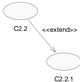
Figure 12: An <<extend>> is a standard UML association represented by an open arrow that points to the use case that is being employed as an extension. An extension increases the behaviour of the base use case
