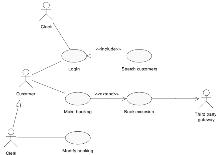
Figure 2: Actor types as part of a hierarchy. The Clerk and Customer are both primary (human) actors. The Third party gateway is a legacy system that accepts excursion bookings. The Clock is an automated convenience that logs users off the system when they have been inactive for a period of time.
