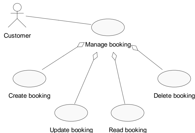
Figure 5: A set of CRUD use cases over the entity booking . The children use cases are shown related to the parent use case via the aggregation relationship.
