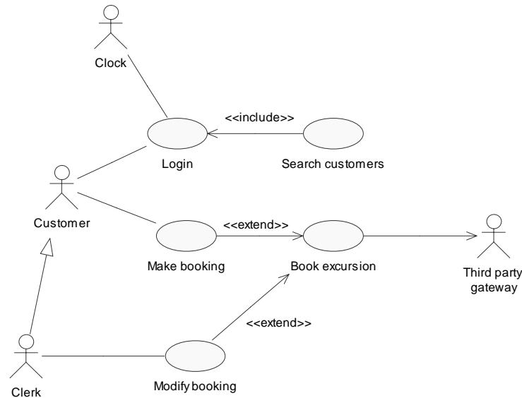
Figure 7: An extract of the total functionality delivered by the booking system.
