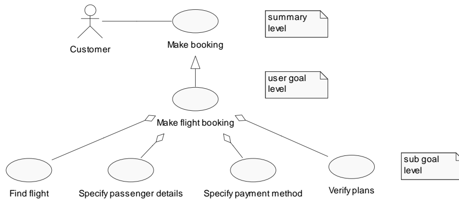
Figure 8: An example of Cockburn’s hierarchy of abstraction of user goals in use cases. Strictly speaking, this type of association between use cases is not defined in the UML specification (staff99). Make flight booking is shown as a specialisation of Make booking . Make flight booking is shown to be comprised of a series of use cases that combine to represent a whole-part relationship.
