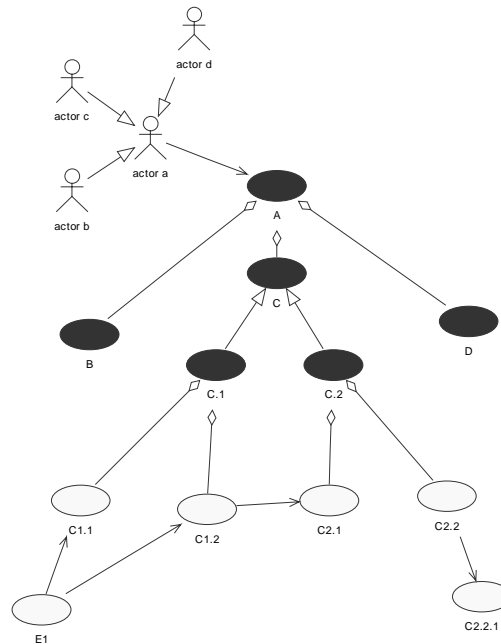
Figure 13: A complex use case model showing four kinds of use case association.
